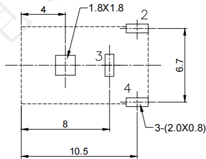
P.C.B LAYOUT VIEW
