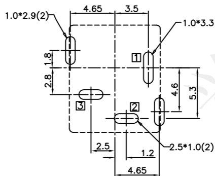
RECOMMENDED P.C.B LAYOUT COPPER-SIDED VIEW ±0.05MM
