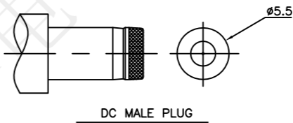
DC MALE PLUG
