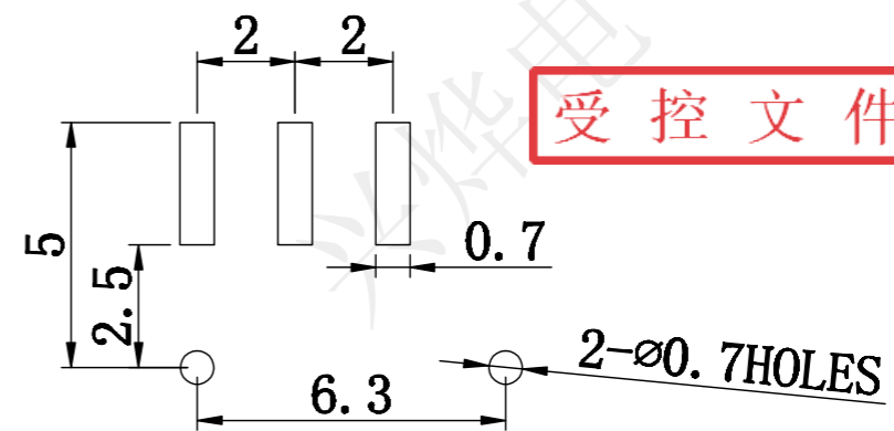
P. C. B LAYOUT DIMENSION
