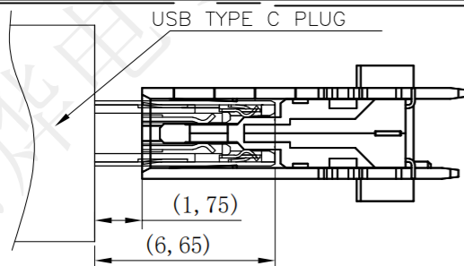
USB TYPE C PLUG
