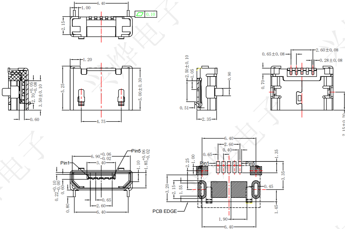
RECOMMENDED PCB LAYOUT PCB图仅供参考
