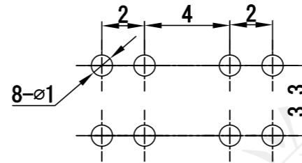
P. B. LAYOUT DIMENSION TOP VIEW
