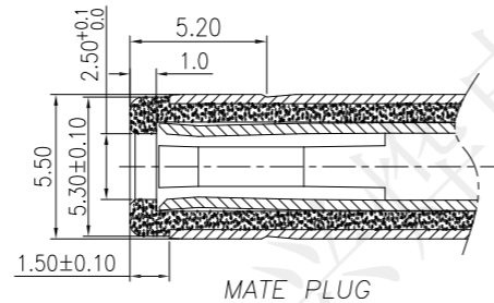
MATE PLUG
