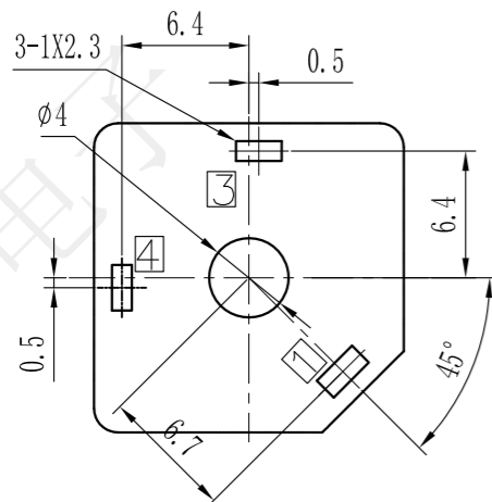
P.C.B LAYOUT (BOTTOM VIEW) Tolerance: \pm 0.05
